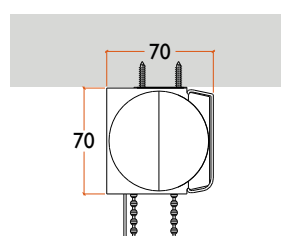
Square Fascia
