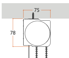
Square Cassette
