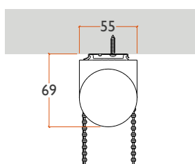
Mounting Profile
