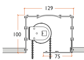
Ceiling Pocket
