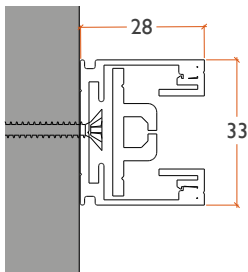
Recess Fix Side Channel
