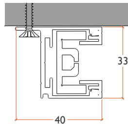
Face Fix Side Channel
