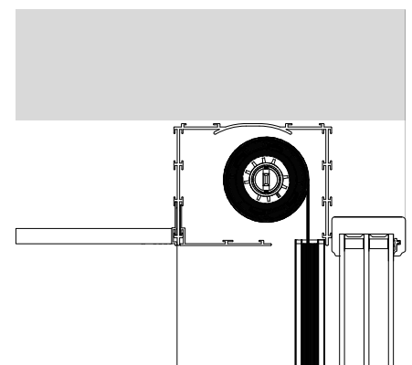
Recess Fix
