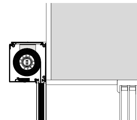
Face Fix
