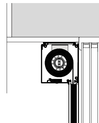
Reveal Fix
